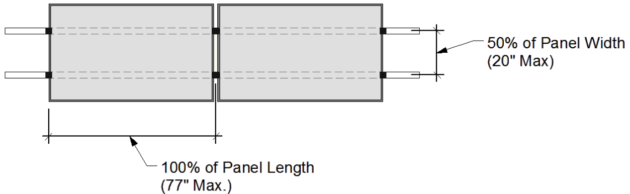
Figure 2 – Proposed Rotated Panel Orientation
