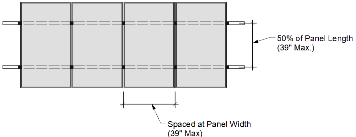
Figure 1 – Currently-Designed Panel Orientation
